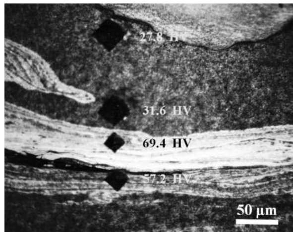
Fig. 12. Measured hardness of the intermetallic layers at the interface.
