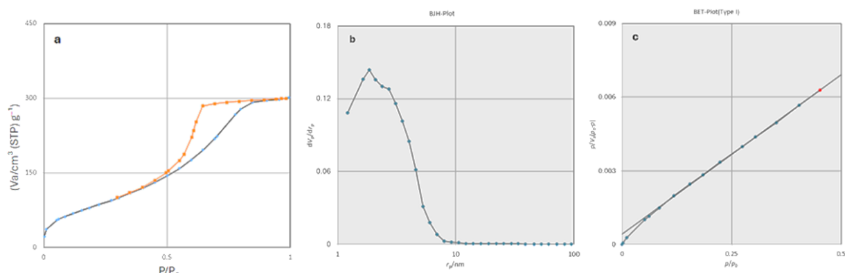
Fig. 7. a) Nitrogen Adsorption-Desorption Isotherm of \text{Fe}_3\text{O}_4@m\text{-SiO}_2 NPs, b) The pore size distribution plot of the \text{Fe}_3\text{O}_4 m-SiO 2 NPs, and c) The BET plot of the \text{Fe}_3\text{O}_4@m\text{-SiO}_2 NPs
