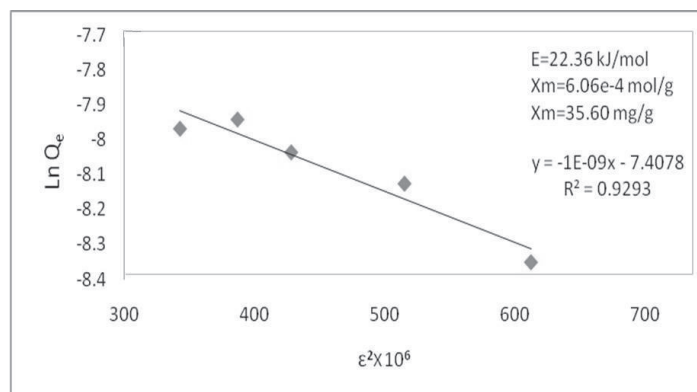
Fig. 6. DKR isotherm for sorption of Ni at 20 °C.
