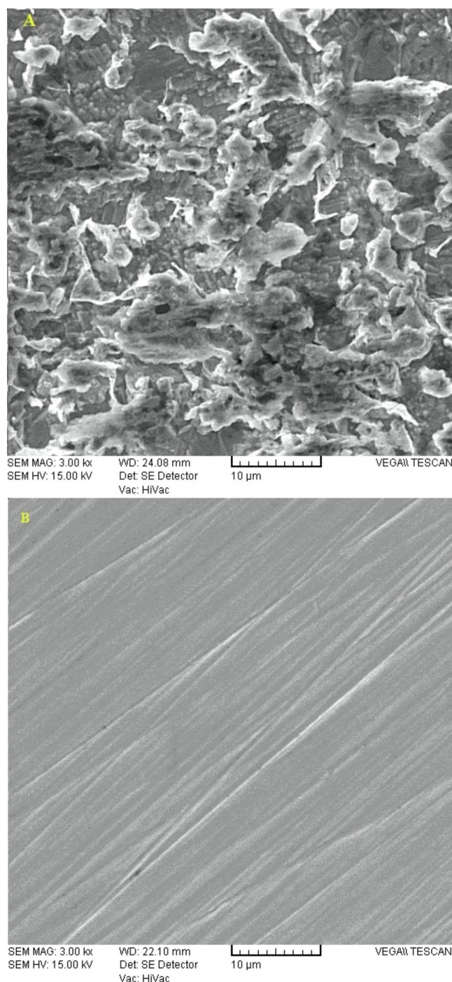
Fig. 9. SEM micrographs of the mild steel surfaces after 48 h immersion period in the blank (A) and 7 \times 10^{-5} M of inhibitor (B) with magnification of 3000.
