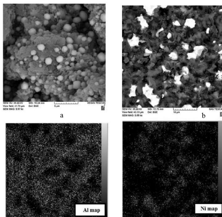
Fig. 6. The SEM micrograph of the two reduced samples at a) at 1300 for 3h, b) at 1650 for 2h, c) corresponding Map of micrograph b
