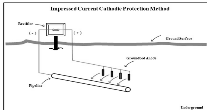
Fig. 1. ICCP Method
