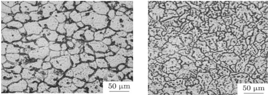
(a) As-weld (before optimizing) (b) Age hardened at 100° C, 8h aging time and 3h solutionizing time(optimized).
