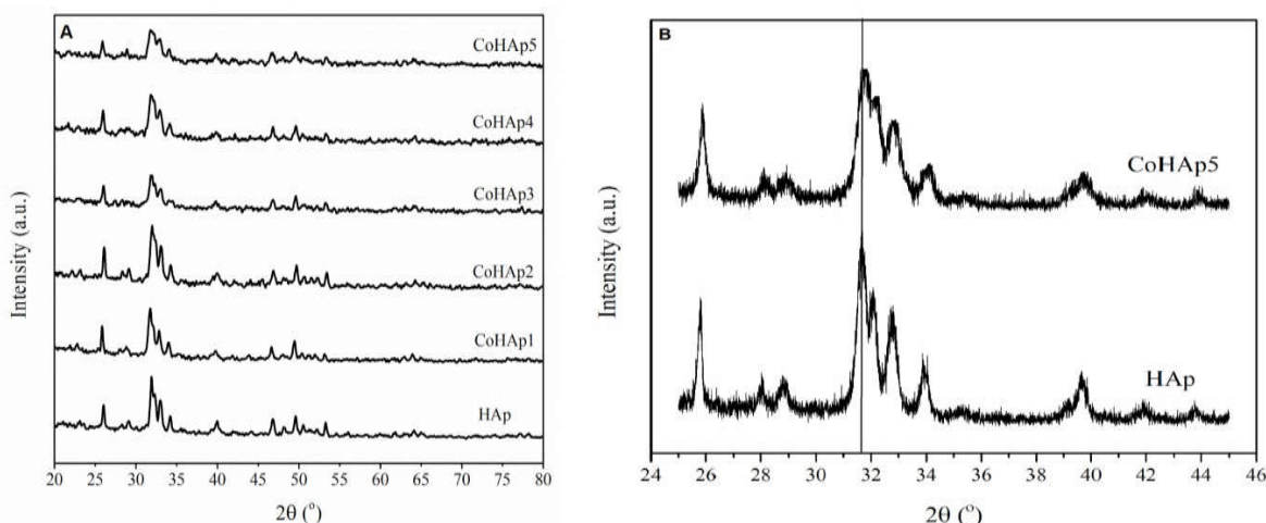
Fig. 1. (A) X-ray diffraction pattern of synthesized HAp, CoHAp1, CoHAp2, CoHAp3, CoHAp4 and CoHAp5 (B) X-ray diffraction pattern of HAp and CoHAp 5 in the 2θ range of 24-46 with step size of 0.005
