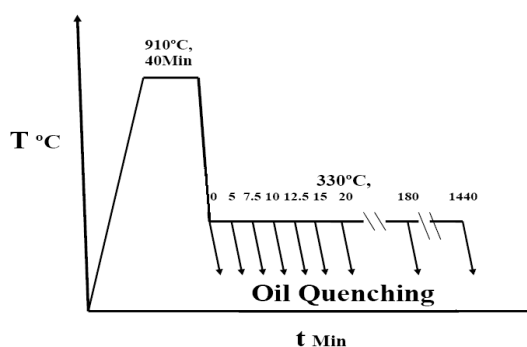
Fig.1. Schematic illustration of heat treatment cycles.
