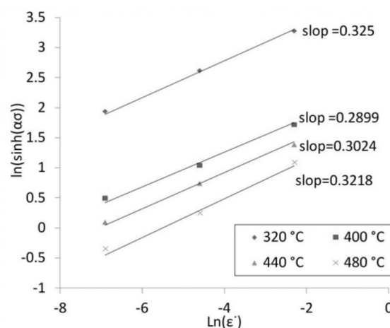
Fig. 5. Isothermal plot of \ln[\sinh(\alpha\sigma)] vs. \ln(\dot{\epsilon}) at various deformation temperatures
