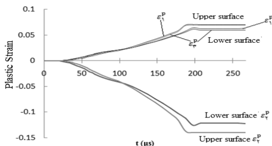
Fig. 15. Components of plastic strain versus time.
