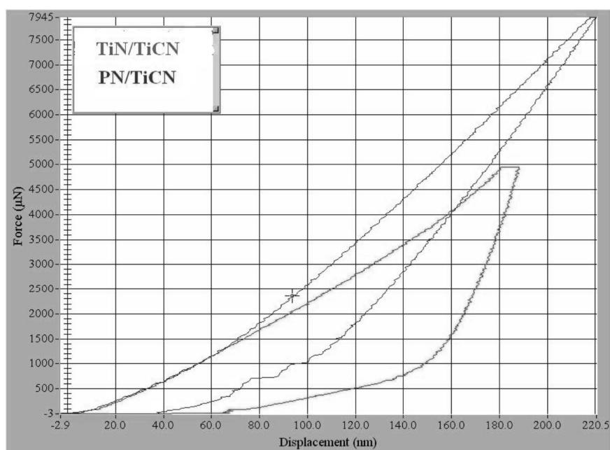
Fig.6. load-displacement curves.
